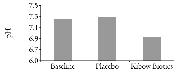
Figure 2. Observed fecal pH values.
